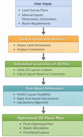
Fig. 2. Workflow of land utilization and automated 2D plan generation module
