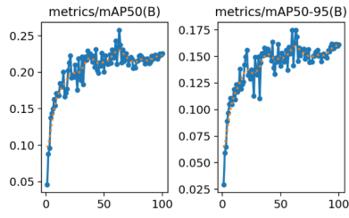
Fig. 9. Mean Average Precision (mAP@0.5 and mAP@0.5:0.95) of the YOLOv8 model for room detection evaluation.
