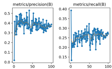
Fig. 8. Precision and recall trends of the YOLOv8 room detection model across training epochs.
