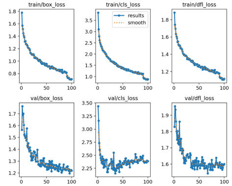
Fig. 7. Training and validation loss curves of the YOLOv8 model for room detection, including box loss, classification loss, and distribution focal loss (DFL).
