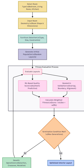
Fig. 4. Workflow of the Interior Space Optimization Module
